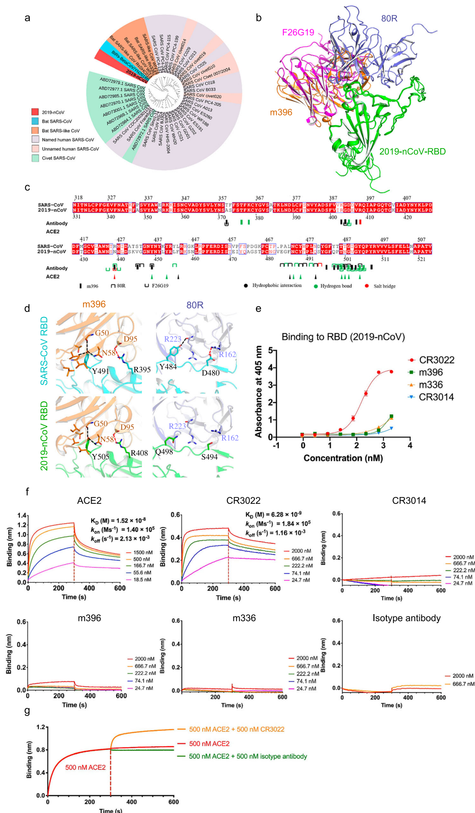
Figure 1. (a) Phylogenetic analysis of 2019-nCoV spike glycoprotein from its protein BLAST sequences. The neighbour-joining tree was constructed using MEGA X, tested by bootstrap method of 2000 replicates, and edited by the online tool of iTOL (v5). (b) The simulated model of 2019-nCoV RBD binding to SARS-CoV-RBD-specific antibodies (m396, 80R, and F26G19). (c) Protein sequence alignment of 2019-nCoV and SARS-CoV RBD, showing the predominant residues that contribute to interactions with ACE2 or SARS-CoV-specific antibodies. (d) The comparison of the complex structures of SARS-CoV-RBD and SARS-CoV-RBD-specific antibodies (shown in the first row) and models of 2019-nCoV-RBD and SARS-CoV-RBD-specific antibodies (shown in the second row). (e) Binding of monoclonal antibodies to 2019-nCoV RBD determined by ELISA. (f) Binding profiles of 2019-nCoV RBD to ACE2 and antibodies, and (g) competition of CR3022 and ACE2 with 2019-nCoV RBD measured by BLI in OctetRED96. Binding kinetics was evaluated using a 1:1 Langmuir binding model by ForteBio Data Analysis 7.0 software.
